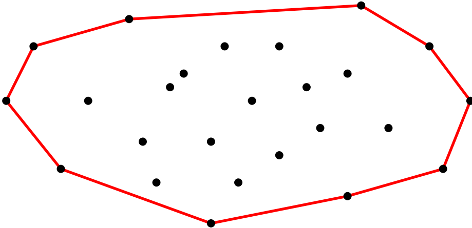
Convex hull
