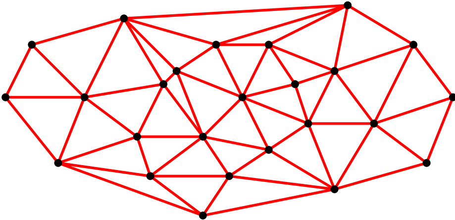
Delaunay triangulation
