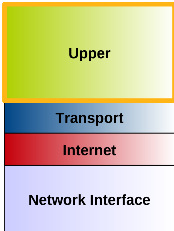
TCP/IP
