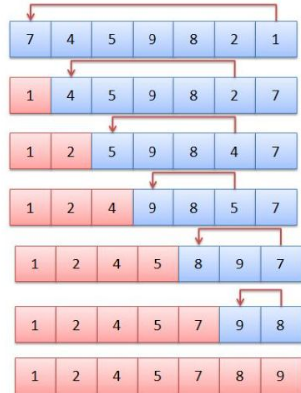
Selection Sort:
